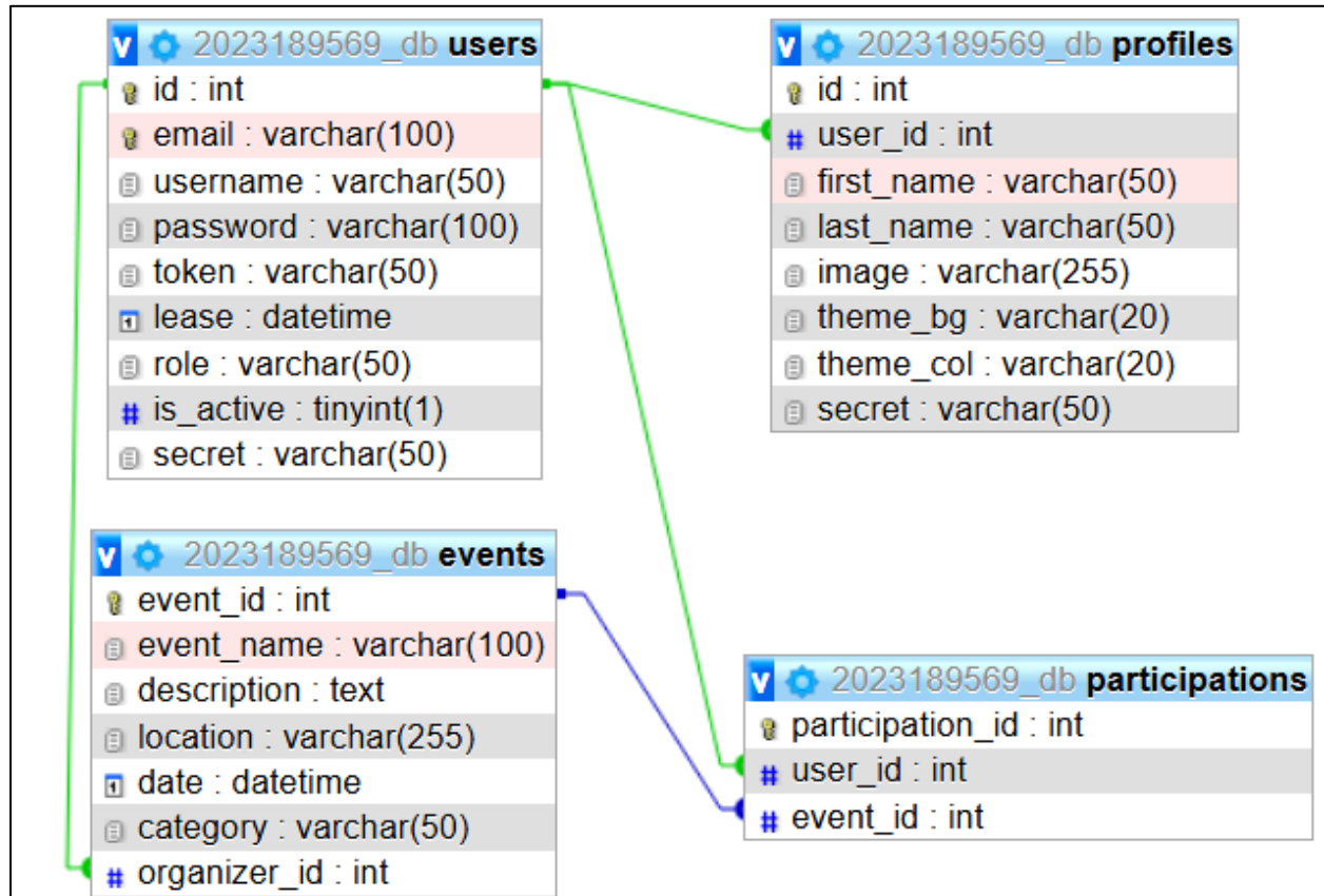
Figure 2.0 ERD Diagram of Social Good Volunteer App
