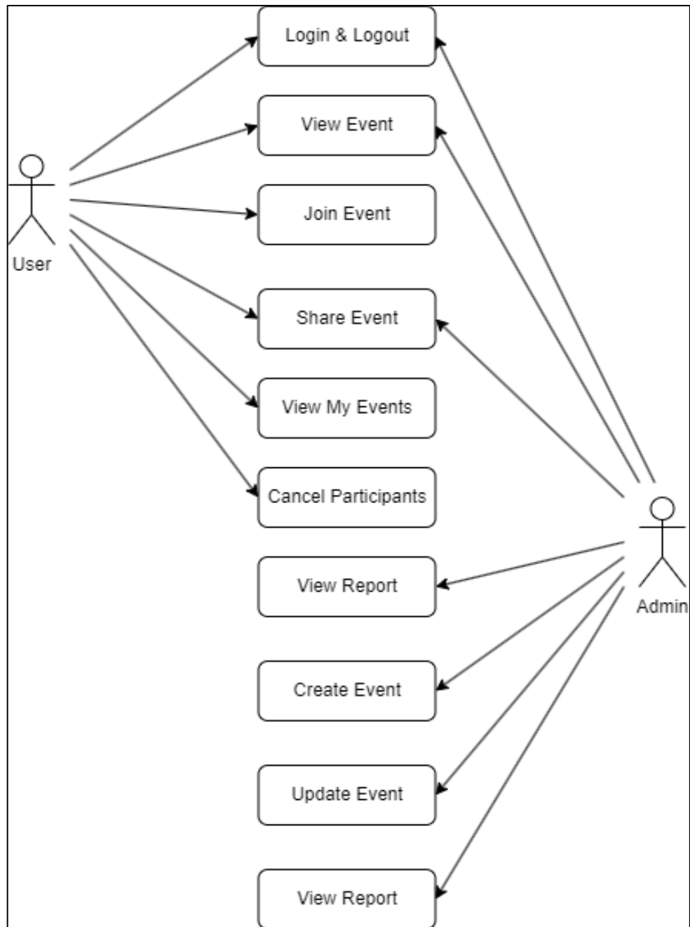
Figure 1.0 Use Case Diagram of Social Good Volunteer App
